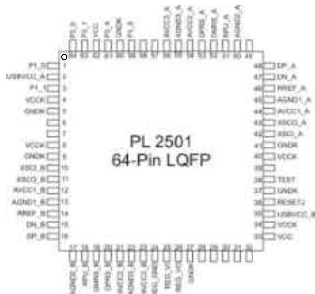
Gambar 2.3 Pinout chip PL 2501 LQFP 64.
