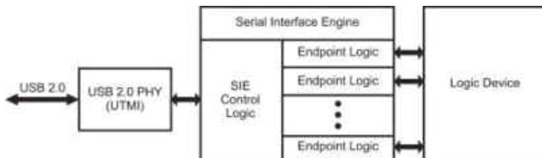
Gambar 4.8 Blok diagram USB Transceiver.
