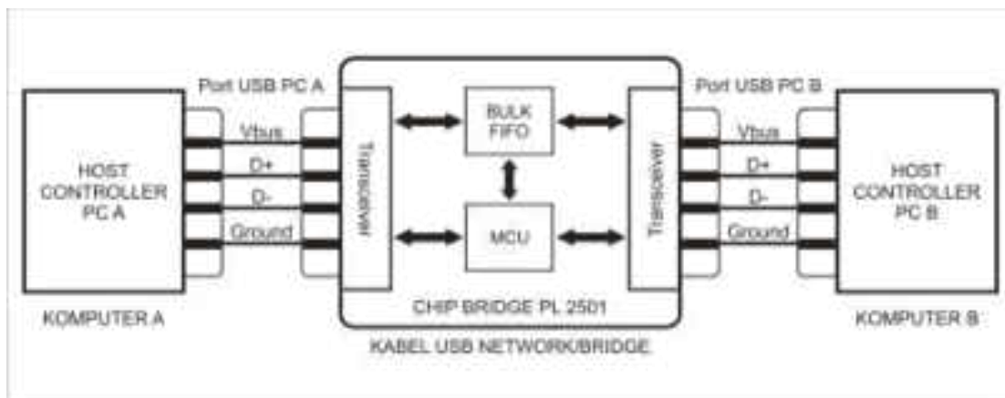
Gambar 4.1. Blok diagram kabel USB Network/Bridge.
