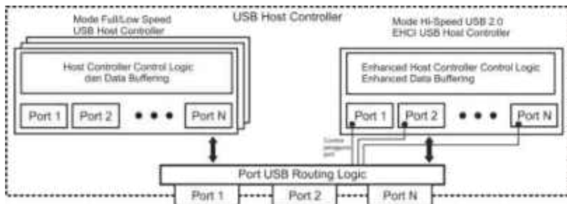
Gambar 4.2. Blok diagram USB Host Controller.
