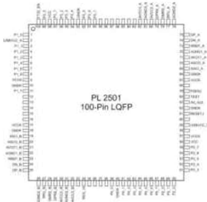
Gambar 2.2 Pinout chip PL 2501 LQFP 100.
